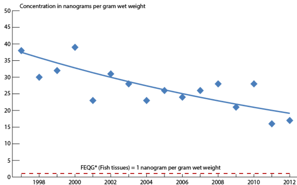
Figure 8. PentaBDE concentrations in Lake Ontario Lake Trout, 1997-2012. Source: ECCC (2017)
