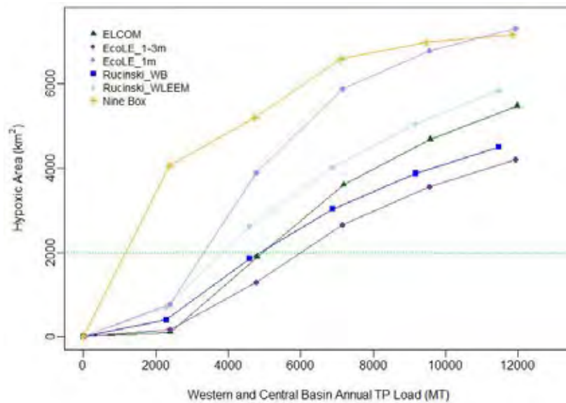
Figure 17. August-September average extent of the hypoxic area predicted by different models in the Central Basin as a function of annual TP loads to the Western and Central Basin. The green horizontal dotted line indicates a suggested threshold of 2000 km 2 .
