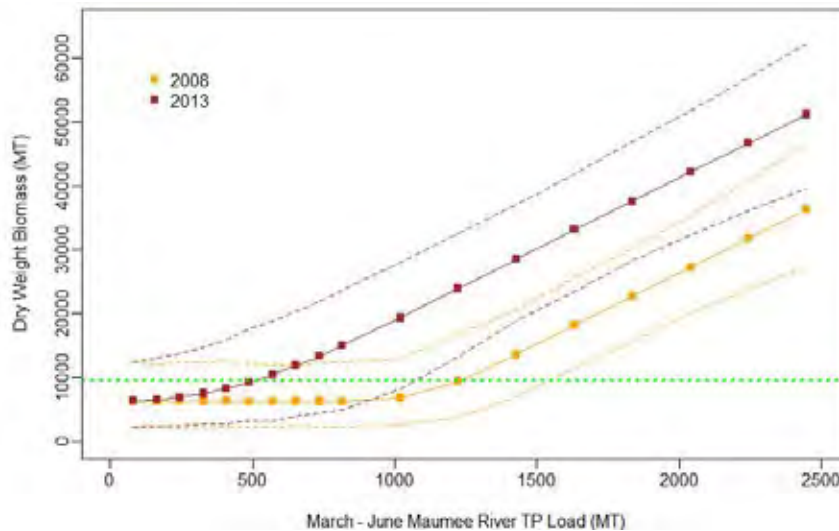
Figure 15. Cyanobacteria bloom size (peak 30-day average biomass) predicted by the Obenour et al. model in the Western Basin as a function of spring Maumee River TP load. Solid lines represent mean predictions under 2008 and 2013 lake conditions (see Appendix B-2 of Scavia and DePinto (2015) for details), while dashed lines represent 95% prediction intervals. The green horizontal dotted line indicates the threshold for “severe” blooms.
