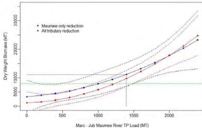
Figure 16. Cyanobacteria bloom size (peak 30-day rolling average biomass) as a function of March – July Maumee River TP load, predicted by WLEEM in the Western Basin in relation to changes in TP loads from all external sources (red lines) and from the Maumee River only (blue lines). Solid lines represent mean predictions, while dashed lines represent 95% prediction intervals around the regression fitted through results of model simulations using 2008, 2011-13 (Appendix B-7 of Scavia and DePinto (2015)). The black dotted line marks the 2008 TP load and corresponding bloom prediction. The green horizontal dotted line indicates the biomass level corresponding to a decrease in the 2008 bloom prediction equivalent to the percentage reduction of Stumpf’s 2008 predicted value down to the satellite data based value of 9600 MT. To account for this difference in calculation of this 30-day biomass value and to provide a bloom threshold consistent with WLEEM’s biomass estimates and equivalent to 9600 MT, we calculated the ratio of the Stumpf modeled 2008 biomass (our baseline year and also a severe bloom year) to the 9600 MT value, and then applied that ratio to the 2008 biomass predicted by WLEEM to obtain an “equivalent” threshold of 7990 MT cyanobacteria biomass for WLEEM (green line).
