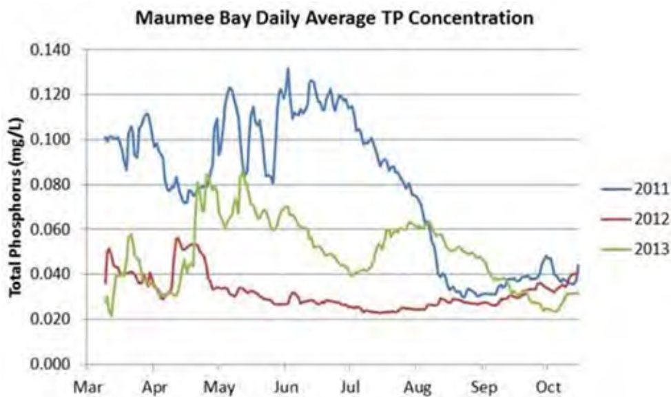
Figure 21. Maumee Bay daily average TP concentration simulated by WLEEM for 2011, 2012, 2013.
