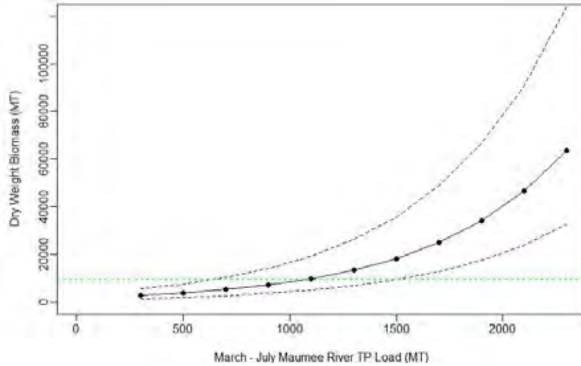
Figure 14. Cyanobacteria bloom size (peak 30-day average biomass) predicted by the Stumpf et al. (2012) model in the Western Basin as a function of spring Maumee River TP load. The solid line represents mean predictions, while dashed lines represent 95% prediction intervals. The green horizontal dotted line indicates the threshold for “severe” blooms.
