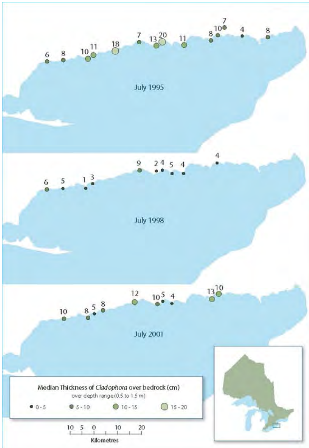
Figure 23. Median thickness of Cladophora growing over bedrock on the north shore of the Eastern Basin of Lake Erie. Figure extracted from Ontario Ministry of Environment Water Quality in Ontario report for 2008.
