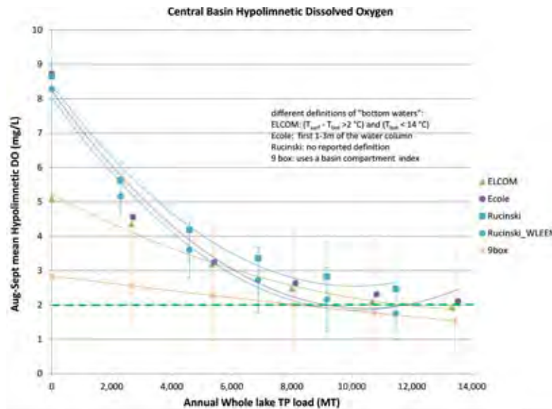
Figure 18. August-September average hypolimnetic dissolved oxygen concentration predicted by different models in the Central Basin as a function of annual TP loads. The green dotted line shows the annual whole-lake load to achieve a threshold of 2 mg/L for the various models.
