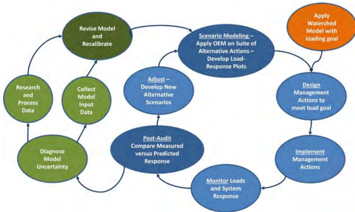
Figure 22. Adaptive management process employing an Operational Ecosystem Model (after DePinto 2013).
