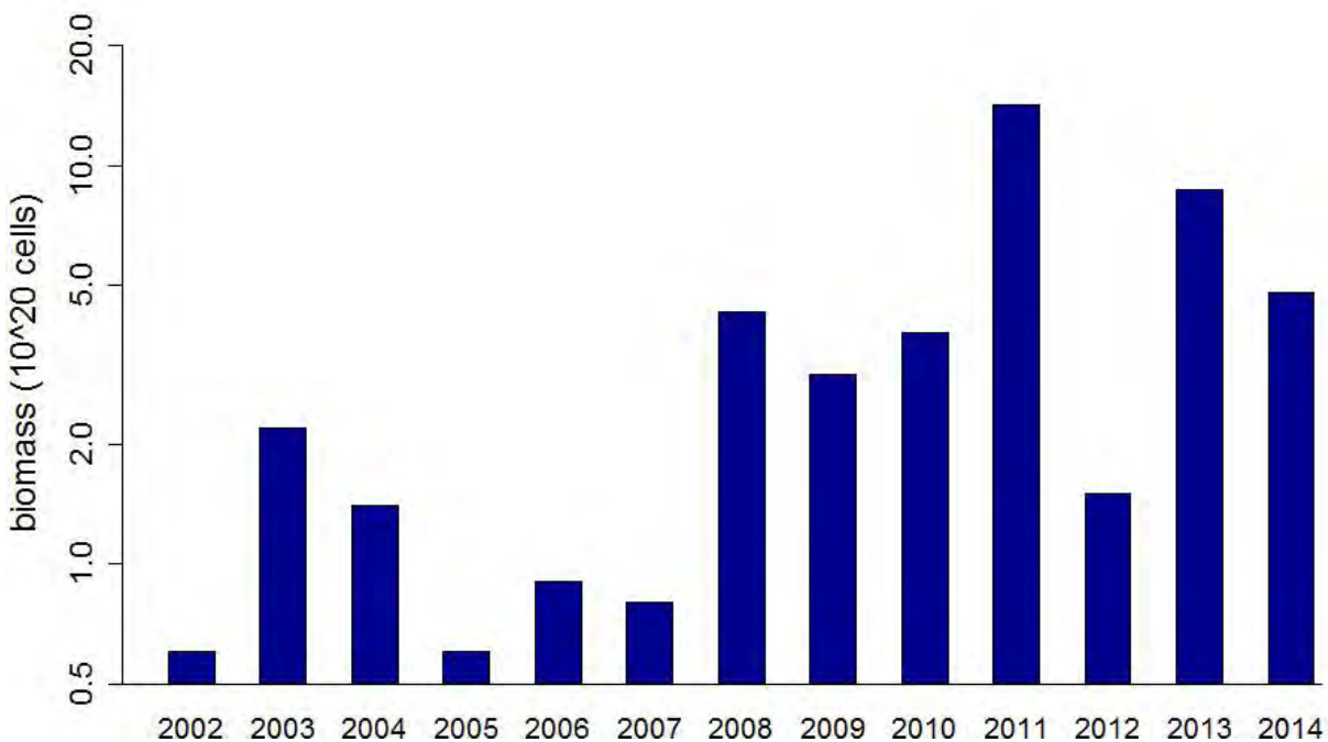
Figure 3. Cyanobacterial biomass for western Lake Erie based on measurement from satellite. (Stumpf personal communication, updated from Stumpf et al. 2012)
