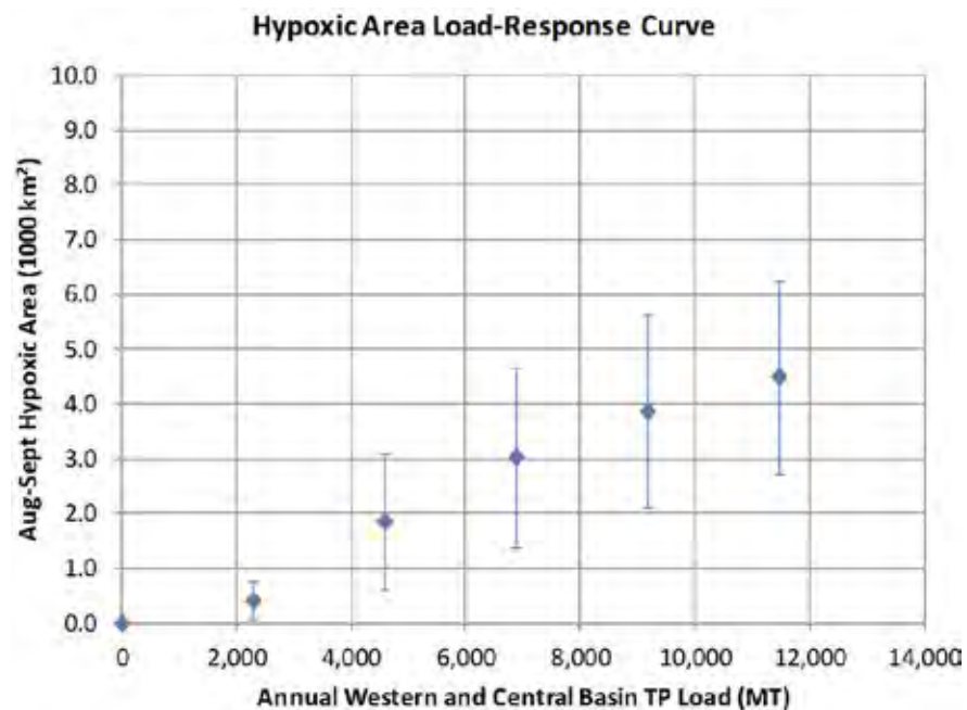
Figure 20. Aug-September average hypoxic area load-response curve computed by Rucinski 1D Hypoxia Model. Mean of 1987-2005 model estimates values shown as blue diamonds. Standard deviation of 1987-2005 values shown as vertical error bars.
