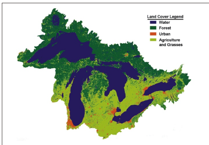
Land cover type and distribution in the Great Lakes basin in the 1990s.
